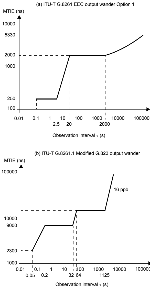
Figure 13 (a) ITU-T G.8261 EEC output wander option 1. Applies to the output of an EEC-1 but also may apply to a PEC-M and PEC-S. (b) ITU-T G.8261.1 modified ITU-T G.823 mask that applies to PEC-S output.
