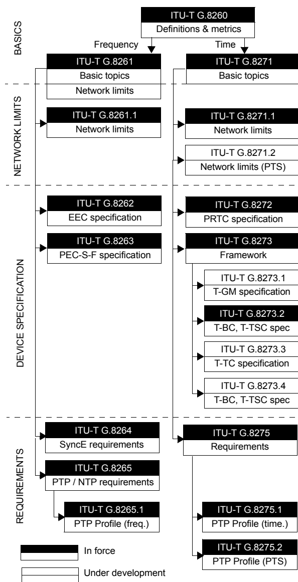
Figure 1 ITU-T packet switched network synchronization standards and the relationship among them.
